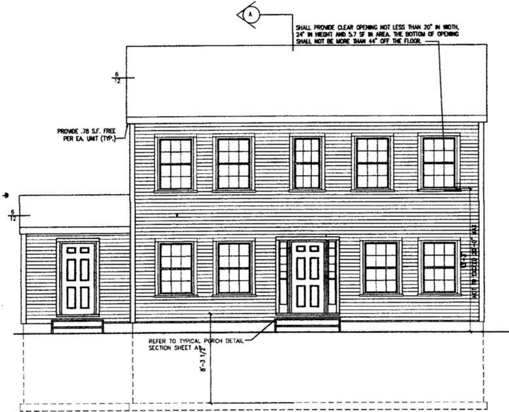
FRONT ELEVATION
