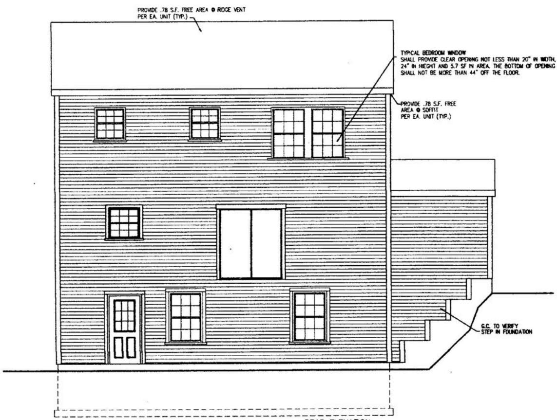
REAR ELEVATION
